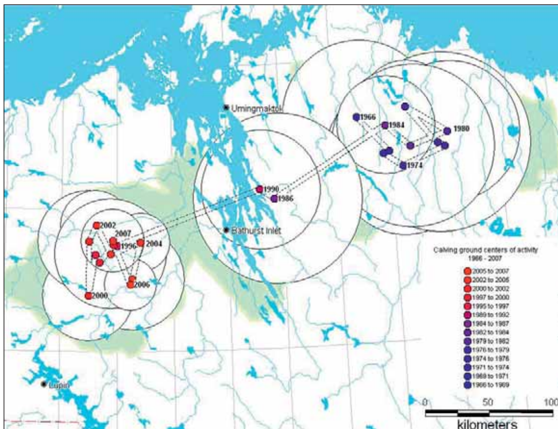
Fig. 2. Centroids of annual calving grounds at the peak of calving for the Bathurst herd, 1966 to 2007. The centroids are embedded in circles that are equivalent to the area of the annual calving ground; larger circles denote larger annual calving grounds (see Gunn et al. , 2008 for further explanation).
