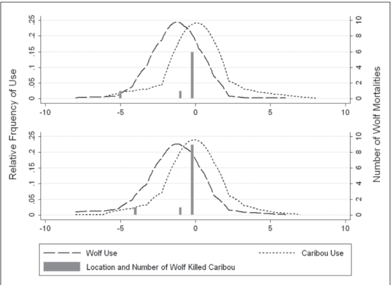
Fig. 2. Seasonal overlap of caribou and wolves showing relative probability of use as a function of the difference between summer (top) and winter (bottom) caribou and wolf resource selection models, and location and frequency of caribou mortalities (black bars). Note the X axis is the difference between binned RSF values of caribou and wolves, such that high values (10) represent safe areas for caribou, and low values (-10) represent high wolf use areas.
