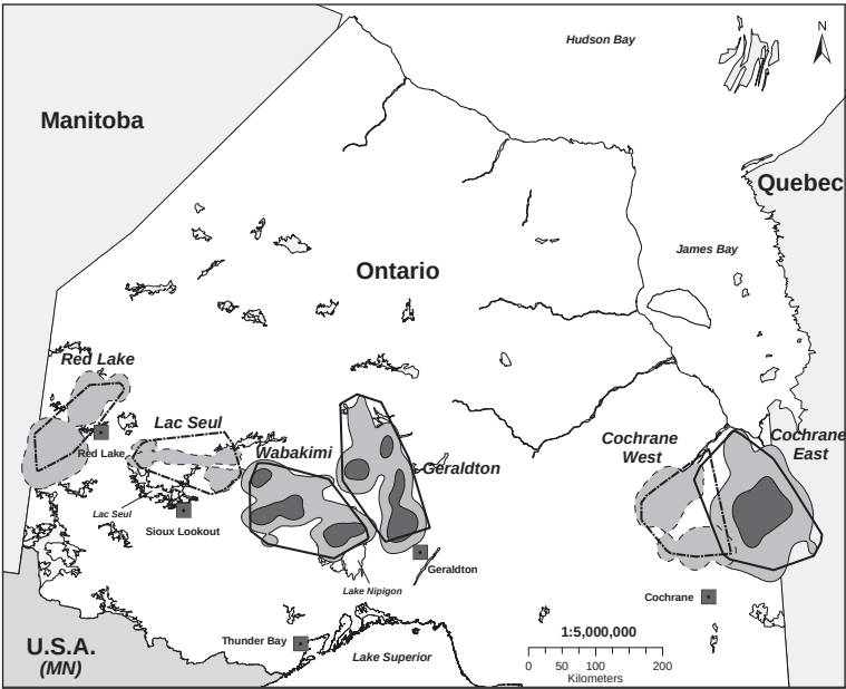
Fig. 5. Demographic unit boundaries and core areas of forest-dwelling woodland caribou ( Rangifer tarandus caribou ) at the southern limit of the ecotype's continuous distribution in Ontario. Angular polygons outlined in black represent 100% Minimum Convex Polygons generated using all the subsampled locations of the caribou assigned to each cluster. Light gray polygons represent boundaries defined using the 95% isopleth from kernel density estimates of the utilization distributions for caribou assigned to each cluster. Polygons with dashed outlines were generated using location data from a small sample of individuals. Isopleths generated using data from relatively large, broadly distributed samples of individuals have solid outlines (i.e., Wabakimi, Geraldton and Cochrane East clusters), while isopleths generated using data from a small samples of individuals have dashed outlines (i.e., Red Lake, Lac Seul, Cochrane West). Dark gray polygons represent core areas defined using the 50% isopleth from cluster-specific kernel density estimates of the utilization distribution. These core areas were only generated for clusters with large, well-distributed samples of individuals (i.e., Wabakimi, Geraldton and Cochrane East).
