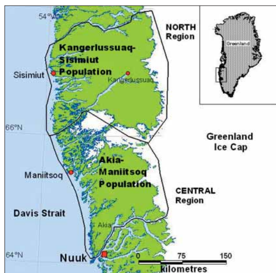
Fig. 1. Regions for the Kangerlussuaq-Sisimiut and Akia-Maniitsoq caribou herds in West Greenland, elevations are not shown.
