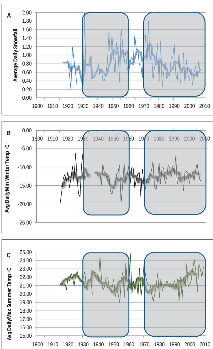
Fig. 4. A) Snowfall, B) average daily minimum winter temperature, and C) average daily maximum summer temperature for Jasper National Park 1900-2009. Grey polygons represent eras within which wildlife abundance trends were consistent. Thick lines depict five year running averages.
