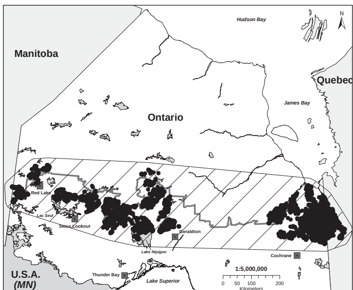
Fig. 1. Study area and locations of sampled individuals. Hatched polygon delineates the general study area, defined by a buffered (25 km) 100% Minimum Convex Polygon. Black circles represent all sub-sampled locations recorded from 1995–2008, for the 73 woodland caribou ( Rangifer tarandus caribou ) included in our analyses. Thick gray line depicts the northern boundary of commercial logging during the time period when location data were collected.
