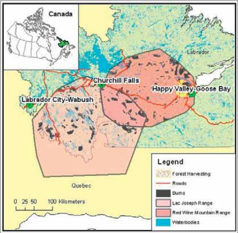
Fig. 1. Range boundaries of the Lac Joseph and Red Wine Mountain caribou populations.
