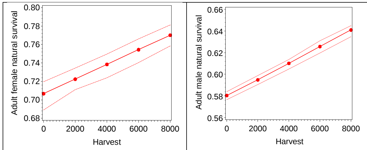
Figure 31. Estimated natural survival for adult females and males under a range of harvest levels. Harvest levels assume 65% cow/35% bull ratio of harvested caribou with demographic parameters from the OLS model. 95% confidence limits on survival estimates are given as dashed lines.
