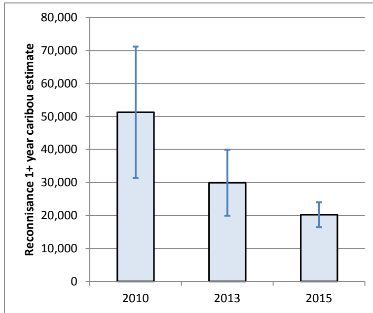
Figure 25: Reconnaissance estimates of caribou on the core calving area.
