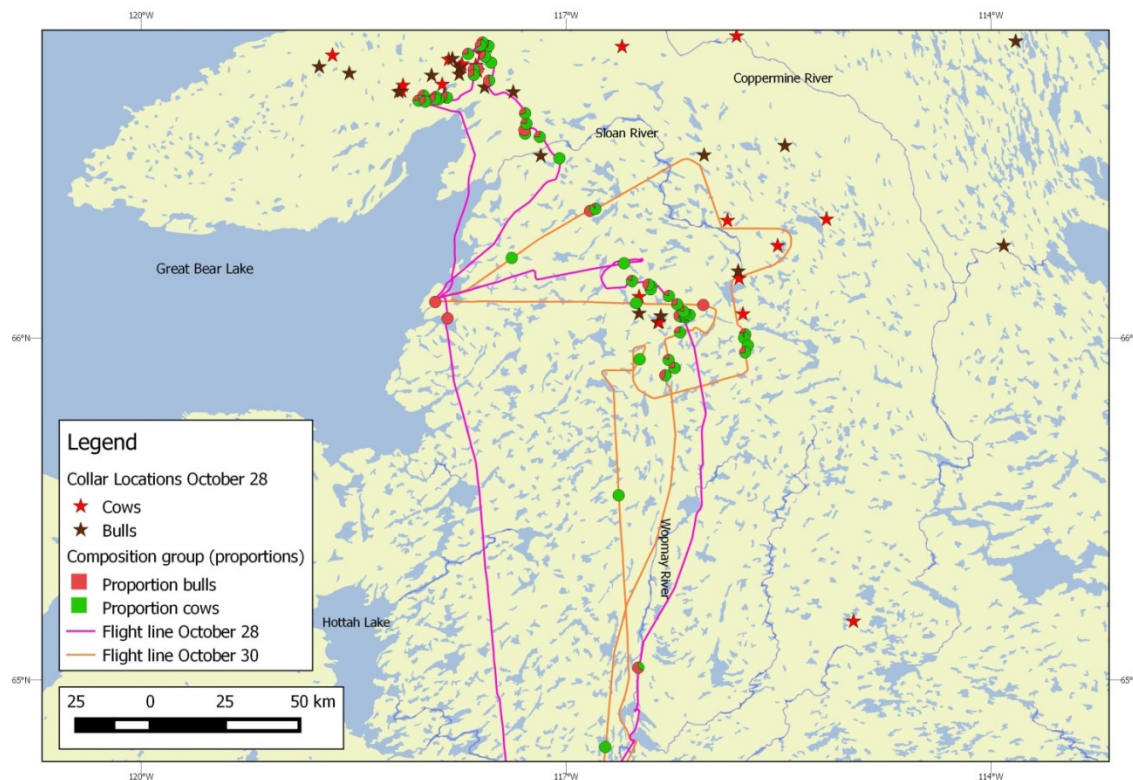
Figure 20. Flight path and groups sampled for fall 2015 composition survey conducted from October 28-30, 2015. Pie charts are given as data points to show proportion cows and bulls observed.
