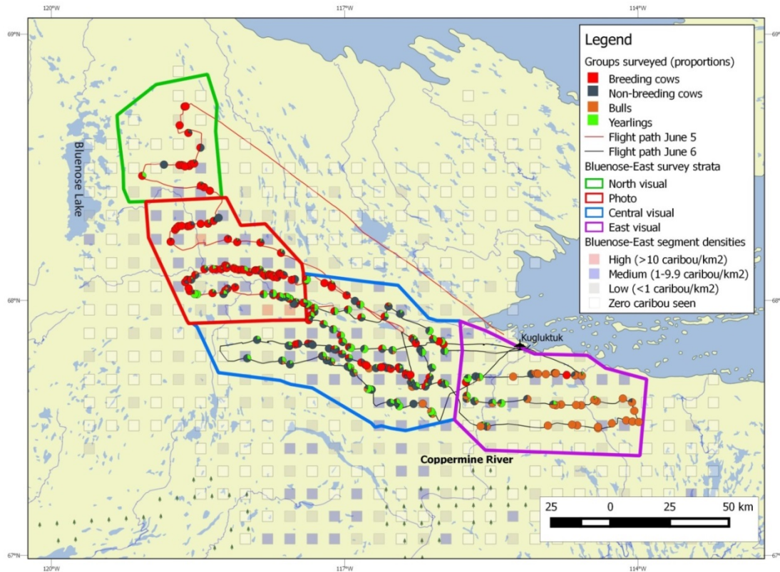
Figure 19. Sampling of composition on the Bluenose-East calving ground from June 5 th and 6 th . Individual sample points are given as pie charts that reflect proportions of the main composition classes in each group sampled. Reconnaissance-based segment densities are given for reference.
