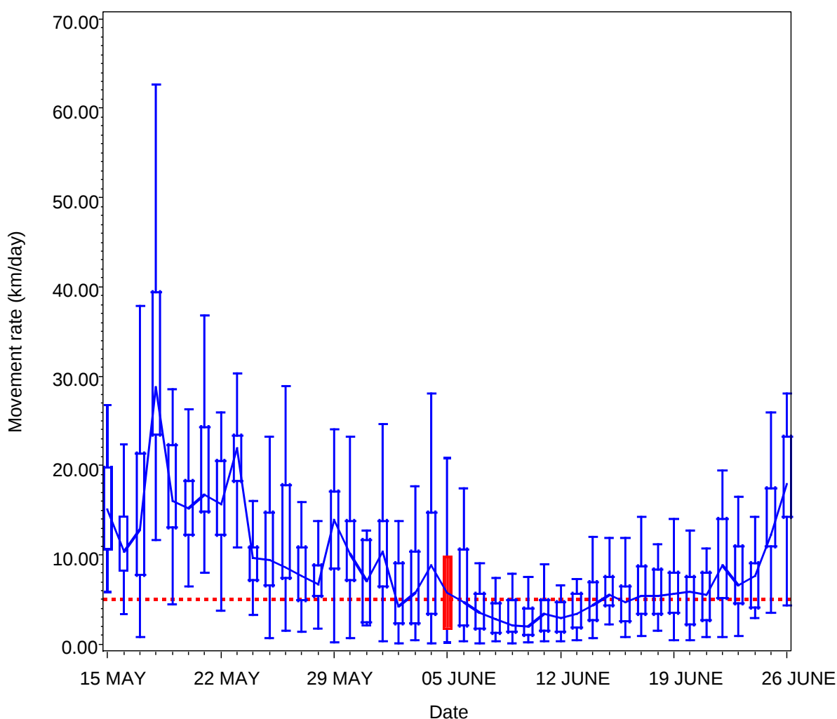
Figure 9. Movements of female collared caribou to the calving ground in 2015. The date (June 5 th ) the visual and photo survey was conducted in highlighted in red.
