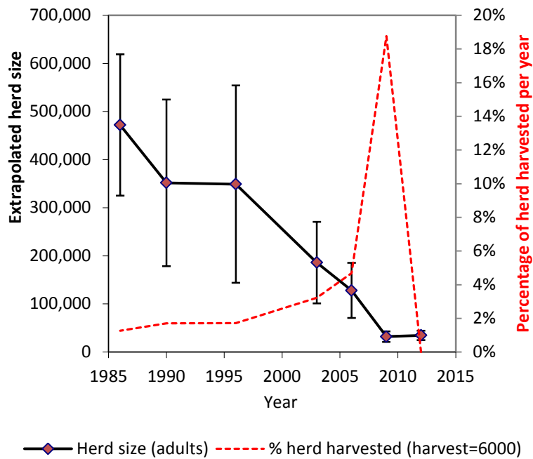
Figure 32. Extrapolated herd size of the Bathurst caribou (left axis) and estimated proportion of the population harvested (right axis) assuming an annual harvest of 6,000 caribou until 2009 and 0 harvest after 2009.
