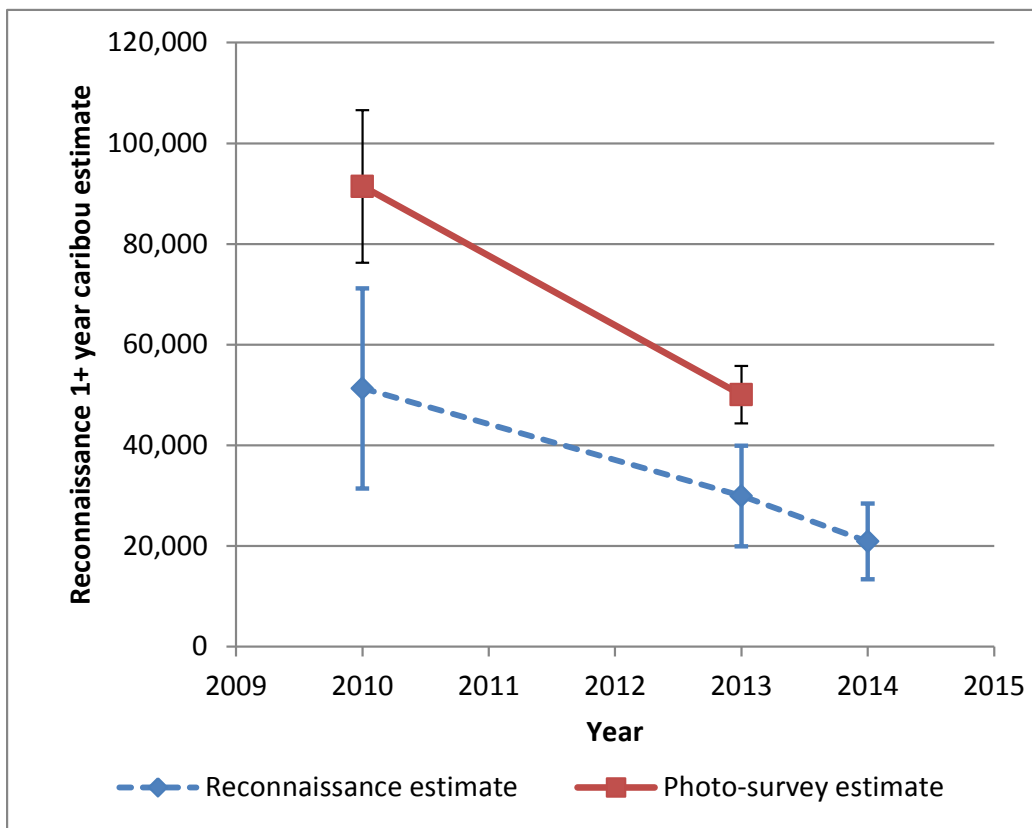
Figure 3. Comparison of estimates of caribou in the core calving area for the Bluenose-East herd from 2010-2014. Estimates of caribou in the core area (not herd size) from the photo plane from surveys in 2010 and 2013 are shown for comparison (red squares). Figure taken from (Boulanger et al. 2014e).
