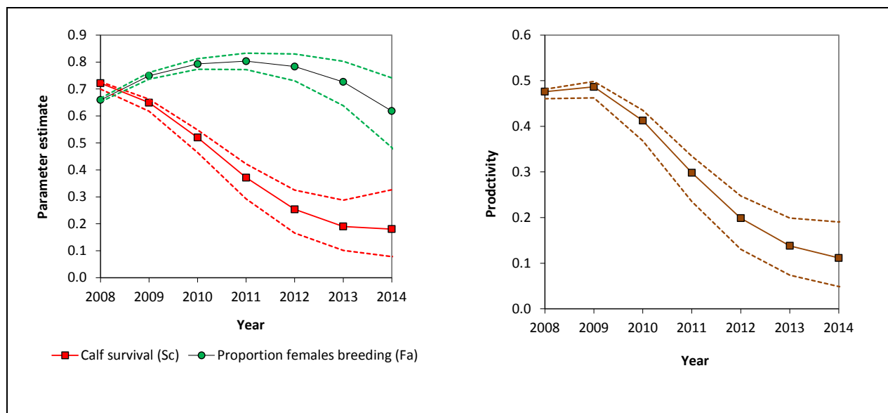
Figure 29. Estimates of calf survival and proportion females breeding from the most supported OLS model (model 1, Table 20). In addition productivity, which is the product of calf survival and proportion females breeding, is displayed.
