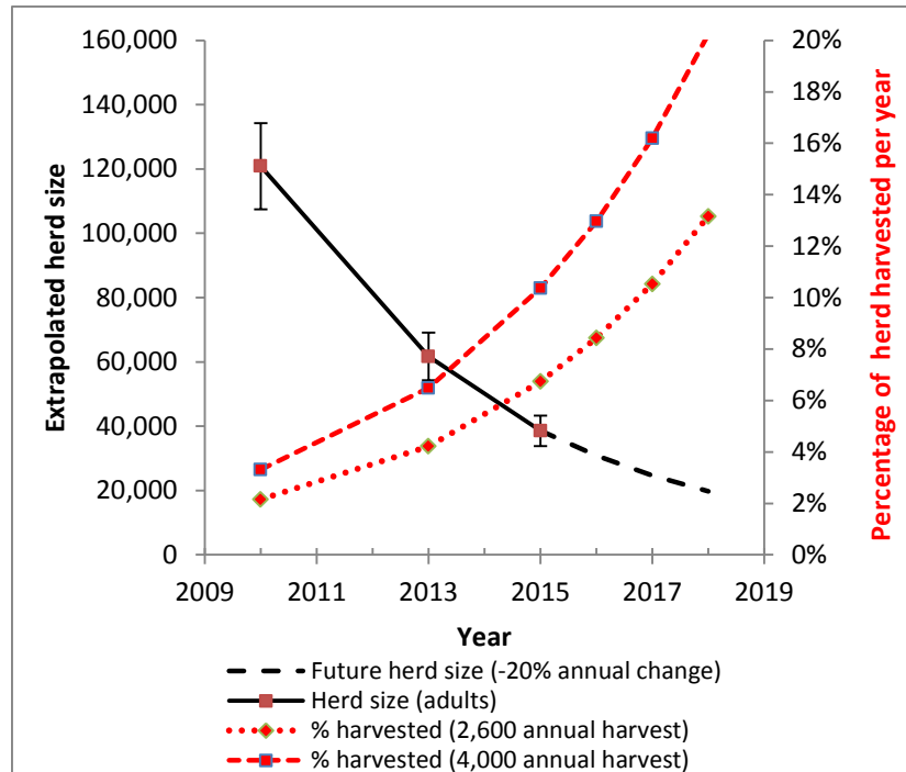
Figure 33. Herd estimates for the Bluenose-East herd and projected herd size assuming the 20% annual decline continues to occur. On the right axis is the proportion of the herd harvested each year under assumed yearly historic harvest levels of 2,600 and 4,000.
