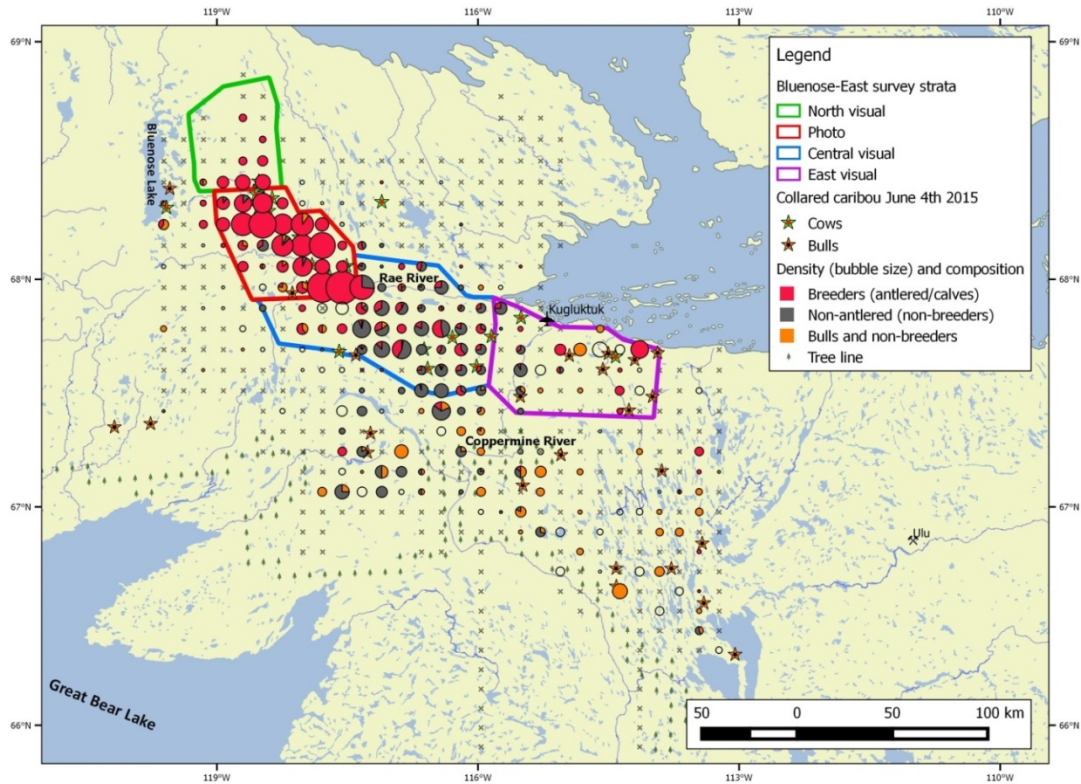
Figure 12. Final strata layout with bubbles representing the relative density of caribou in each segment along with the proportion of breeders classified in the segment. Segments that did not have breeders and non-breeders classified are given as an empty circle (proportional to density) with no colour. Segments with no caribou are shown as an “x”.
