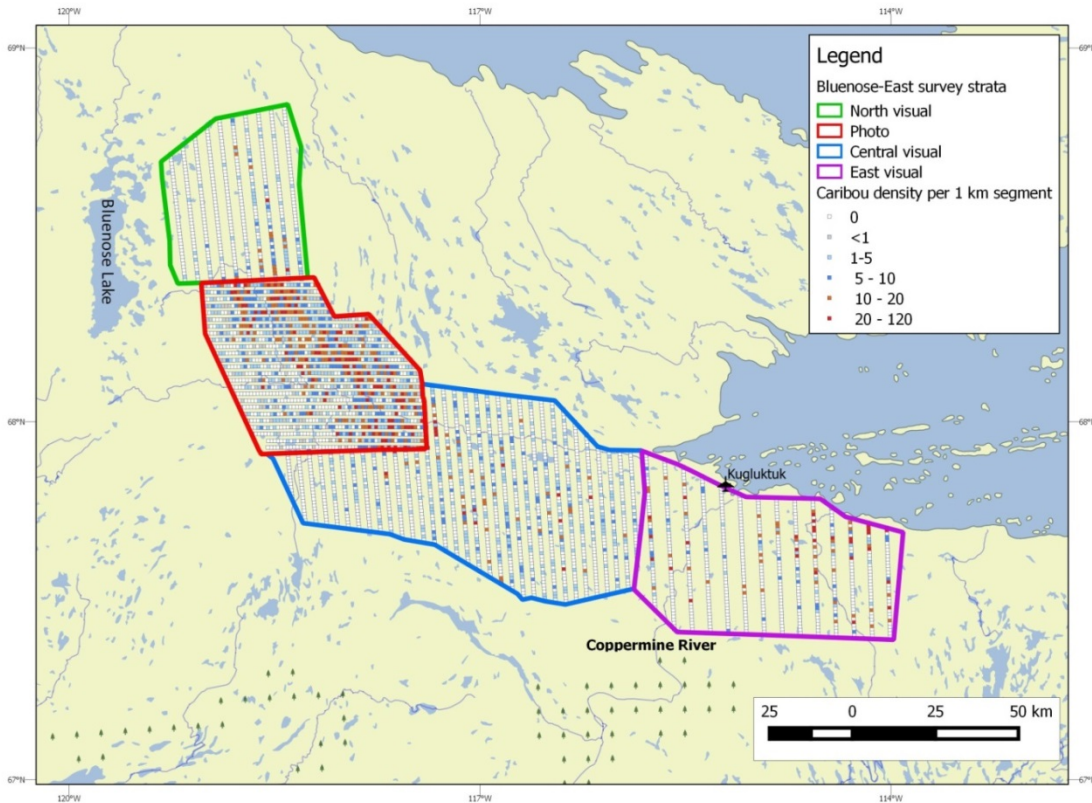
Figure 18. Caribou densities estimated for 1 km transects segments on visual and photo transect lines.
