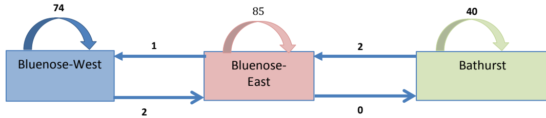
Figure 26. Frequencies of caribou movement events from 2010-2015 based on locations on calving grounds. The arrows above the boxes indicated the number of times a caribou returned to each calving ground for successive years. The arrows indicate movement of caribou to other calving grounds.
