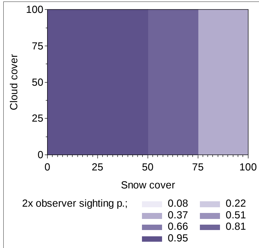
Figure 17. Double-observer sighting probabilities as a function of cloud and snow cover for the Bluenose-East survey.
