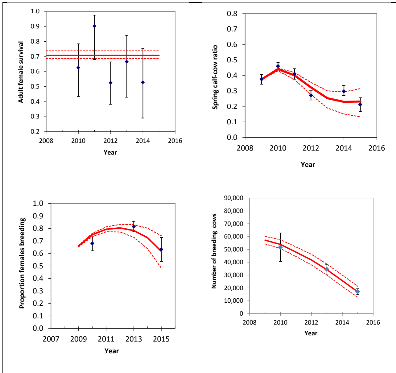
Figure 27. Estimates of adult female survival (from collared caribou), spring calf:cow ratios (from March composition surveys), proportion females breeding and breeding cow (female) population size estimates (from calving ground surveys). Confidence limits are shown on field estimates. OLS model predictions are given as red lines (from model 1, Table 20) with 95% confidence limits on OLS predictions given as dashed red lines.
