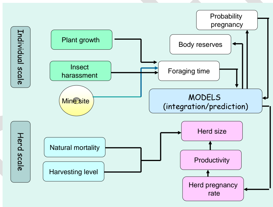
Figure 12. Diagram to illustrate relationships between monitoring at the level of the individual and the herd level, relative to describing cumulative effects.
