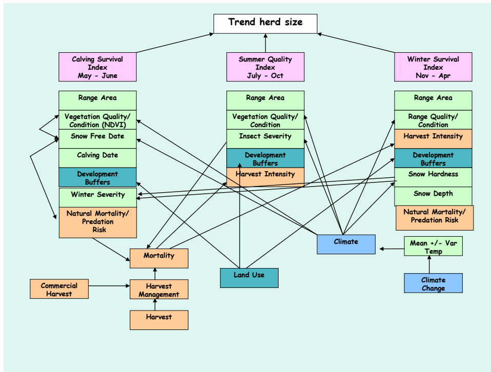
Figure 11. Diagram illustrating known factors influencing caribou health and condition. We have data for the Bathurst herd for most of these, or we can borrow data from other herds.
