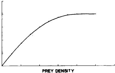
b) FUNCTIONAL RESPONSE NUMBER OF PREY KILLED/PREDATOR
