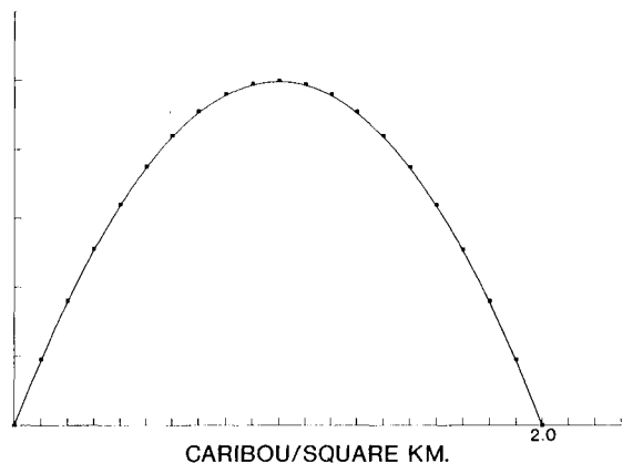
Fig. 1. Annual increment curve for caribou populations in absence of major predators or human harvest.
