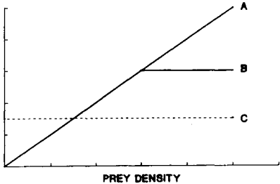
c) NUMERICAL RESPONSE NUMBER OF PREDATORS
