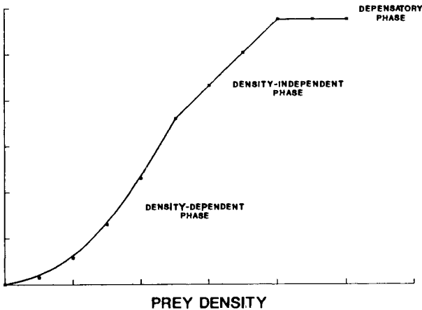
a) NUMBER OF PREY KILLED BY PREDATORS
